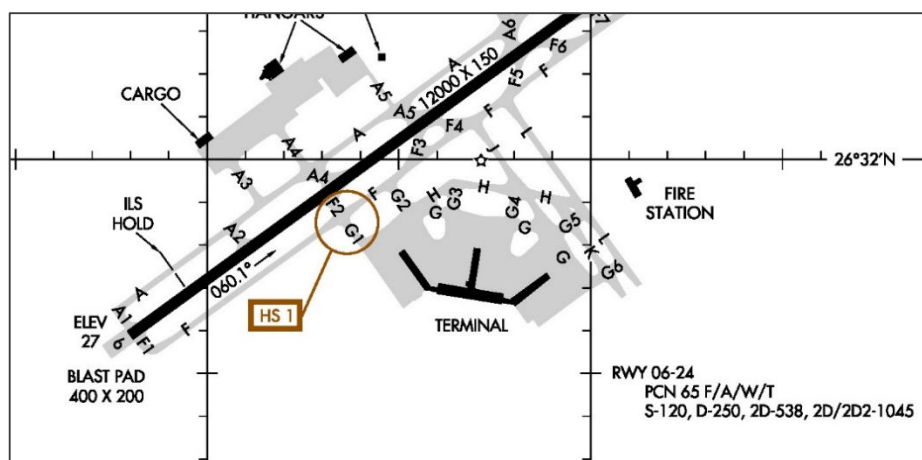
Figure 4-8 Hot Spot 1 at RSW, Taxiway G1
